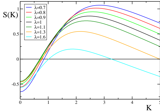
FIGURE 4. (Color online) The dimensionless growth rate S as a function of the renormalized wavenumber K for the slip BC and with an applied electric field. Both the growth rate and K_{fg} increase as the compression increases ( \lambda decreases). Parameters: V = 400V , \Gamma = 0.5 .
