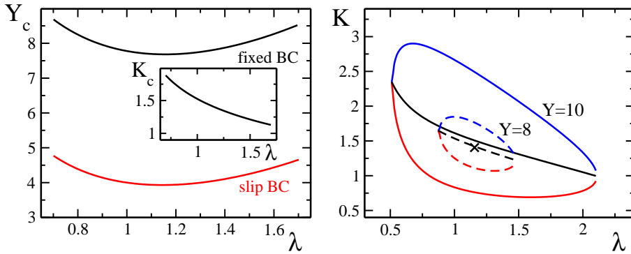
FIGURE 5. (Color online) Comparison of the two BCs at the substrate, for the case of the contactor-induced instability. Left panel: The dimensionless critical Y_c as a function of stretch \lambda for the fixed (black curve) and the slip BC (red). The insert represents the dimensionless critical wavenumber K_c , i.e. the wavenumber that first becomes unstable, as a function of \lambda for the fixed BC; note that for the slip BC, K_c = 0 . Right panel: typical wavenumbers as a function of \lambda for the fixed BC: the fastest growing (black), the minimum and the maximum unstable wavenumbers (red and blue, respectively). For given stretch \lambda , wavenumbers between the red and blue curves will grow. Y = 10 (solid curves), Y = 8 (dashed), the cross marks the position of K_c \simeq 1.40 , where Y_{c,min} \simeq 7.68 and \lambda \simeq 1.156 . Parameter: \Gamma = 0.5 .
