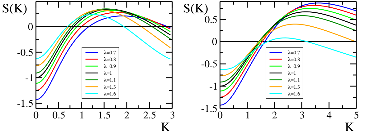
FIGURE 2. (Color online) The dimensionless growth rates of surface undulations, S , as a function of the renormalized wavenumber K for the fixed BC at the bottom. Left panel: case of a contactor ( Y = 10 = \text{const.} ). With increasing compression ( \lambda < 1 ) the wavenumber of the fastest growing mode increases, while it decreases for increasing tension ( \lambda > 1 ). Right panel: case of the capacitor geometry (applied voltage V = 400V ). With decreasing stretch factor \lambda , the fastest growing wavenumber increases. Both figures account for a typical reduced surface tension of \Gamma = 0.5 .
