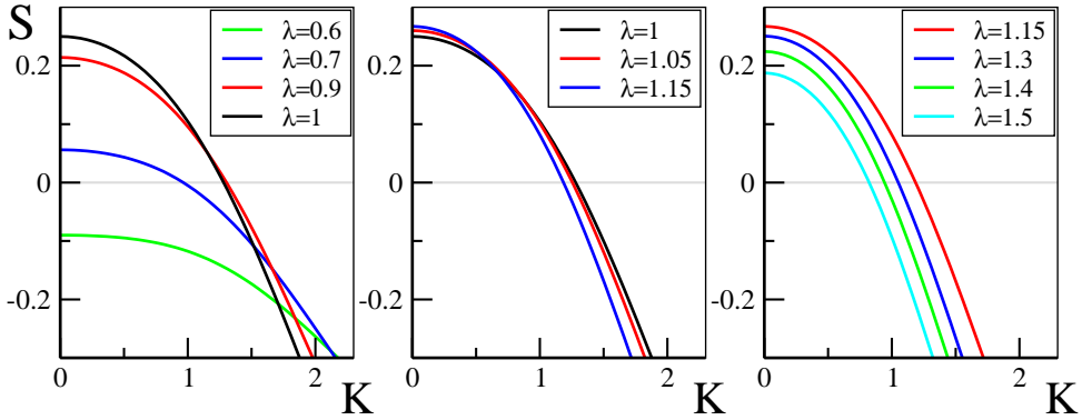
FIGURE 3. (Color online) The dimensionless growth rate of surface undulations, S , as a function of the renormalized wavenumber K for the slip BC and in case of a contactor. The left panel shows increasing compression. For increasing tension, at first the growth rates slightly increase (middle panel), while for higher tension ( \lambda > \lambda_s^* = (\frac{3}{2})^{1/3} \simeq 1.145 ) they again decrease (right). Parameters: Y = 5 , \Gamma = 0.5 .
