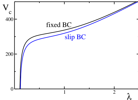
FIGURE 6. (Color online) The critical voltage V_c in the capacitor geometry, as a function of the stretch factor \lambda and for the fixed (black curve) and the slip BC (blue). For an important compression ( \lambda_f < 0.109 and \lambda_s < 0.121 , however beyond the validity of the Neo-Hookean model), buckling-like undulations appear even without an electric field. Both curves show that V_c increases when \lambda increases: a stretch stabilizes the system, while compression destabilizes. The behavior of V_c is quite similar for both BCs; Overall, with the slip BC the system is slightly more unstable. Parameter: \Gamma = 0.5 .
