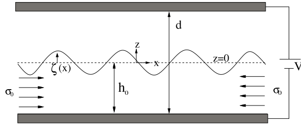
FIGURE 1. Sketch of the capacitor geometry. The thin polymer film is supposed to be under uniaxial stress \sigma_0 in x -direction (which could also be tensile). An external electric field in z -direction (for the unperturbed film) is imposed by externally applying a voltage V between two electrodes a distance d away. The gap can be filled with any dielectric having a differing dielectric constant from the polymer film.
